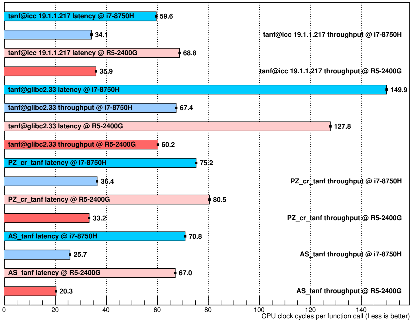
Performance of tanf implementations (10000 random uniformly distributed arguments in [-\pi, \pi] )
