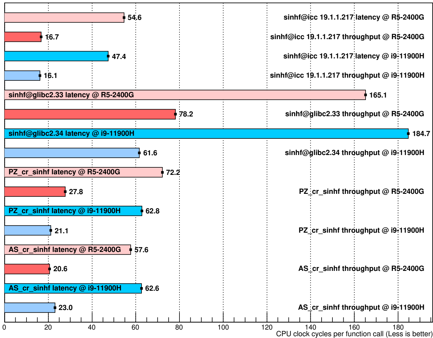
Performance of sinh implementations (10000 random uniformly distributed arguments in [-10, 10])
