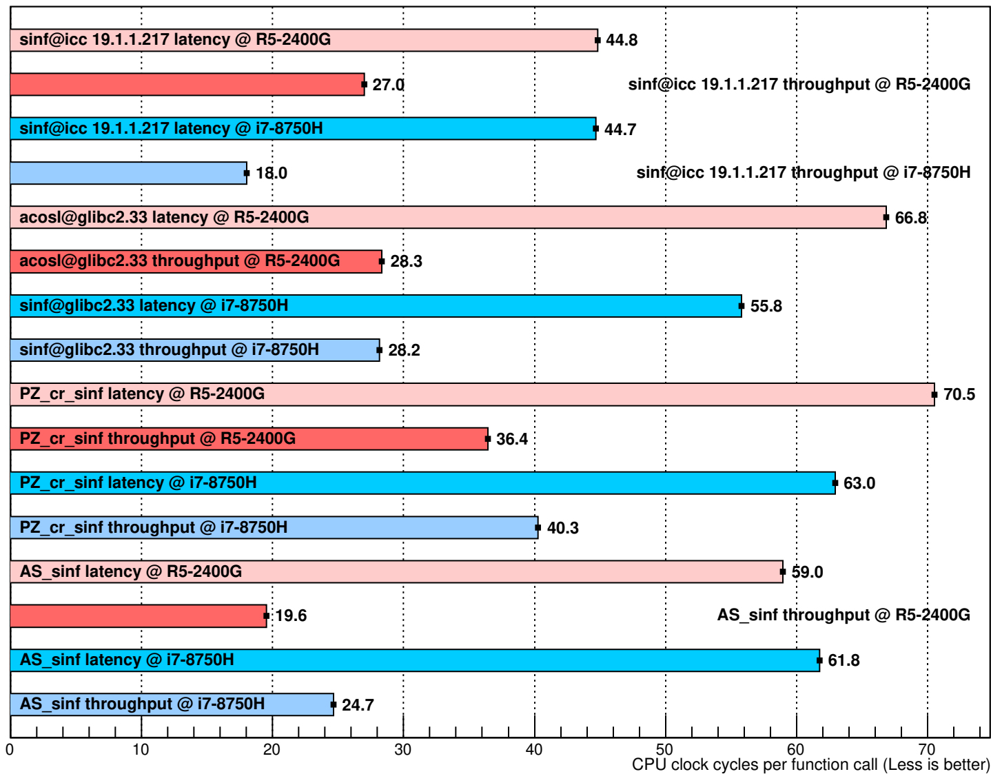
Performance of sinf implementations (10000 random uniformly distributed arguments in [-\pi, \pi] )
