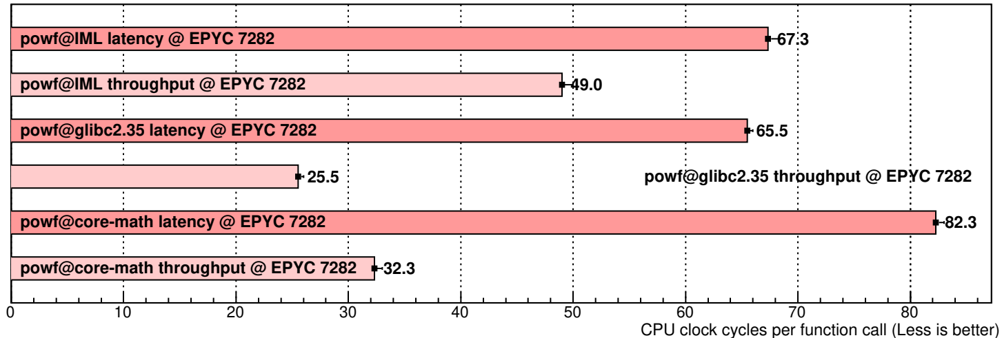
Performance of powf implementations (1000000 random uniformly distributed arguments in [0, 10] \times [0, 10] )
