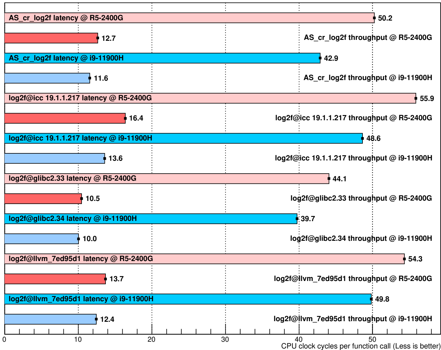
Performance of log2f implementations (10000 random arguments in [e^{-1}, e^{+1}] )
