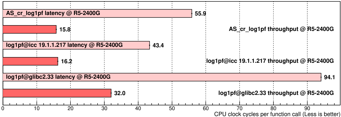
Performance of log1pf implementations (10000 random arguments in [e^{-1/2}-1, e^{+1/2}-1] )
