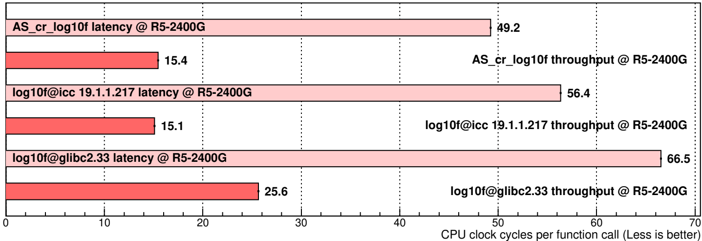
Performance of log10f implementations (10000 random arguments in [e^{-1}, e^{+1}] )
