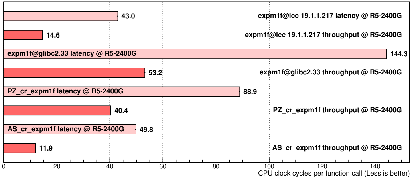
Performance of expm1f implementations (10000 random uniformly distributed arguments in [-10, 10])
