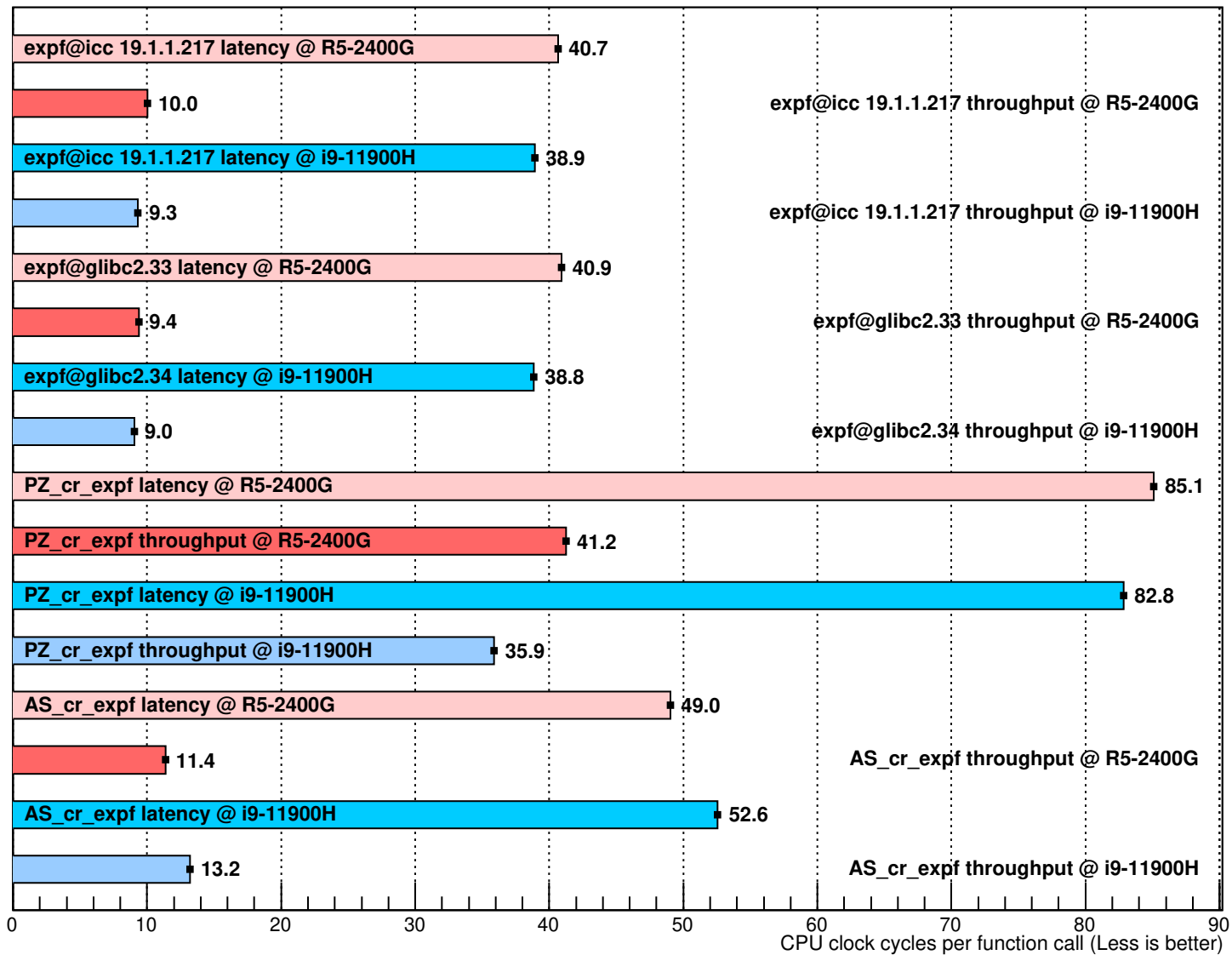
Performance of expf implementations (10000 random uniformly distributed arguments in [-10, 10])
