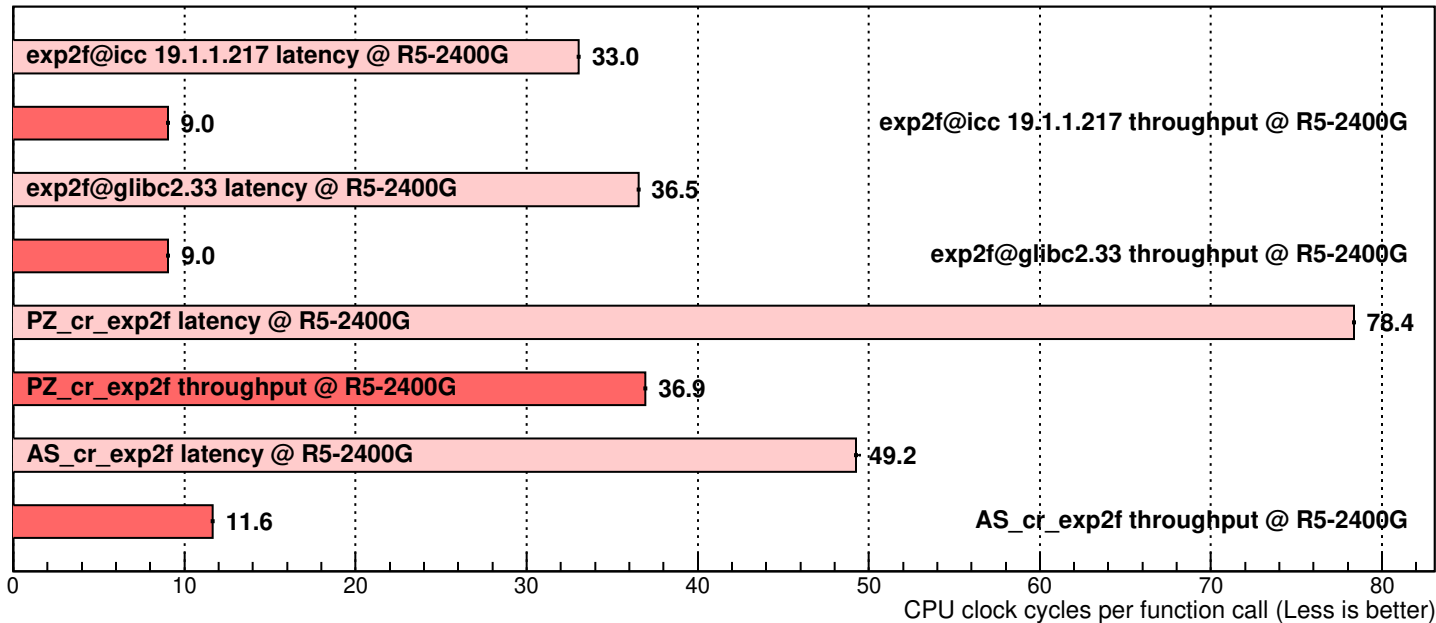
Performance of exp2f implementations (10000 random uniformly distributed arguments in [-10, 10])
