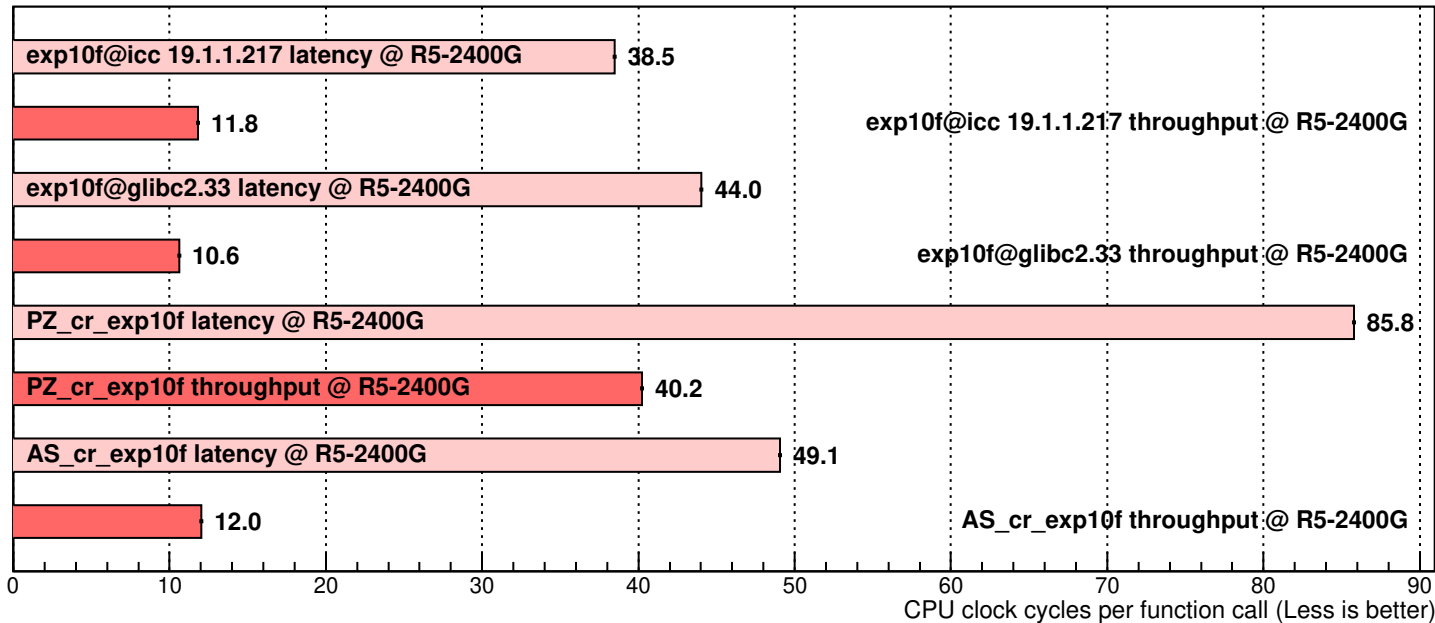
Performance of exp10f implementations (10000 random uniformly distributed arguments in [-10, 10])
