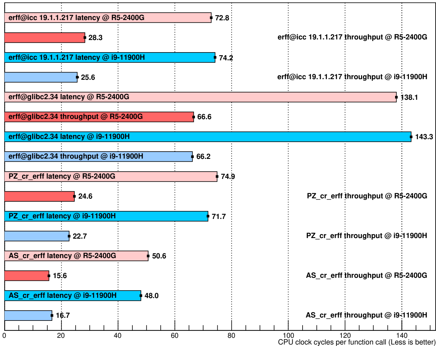
Performance of erff implementations (100000 random uniformly distributed arguments in [-4.16, 4.16])
