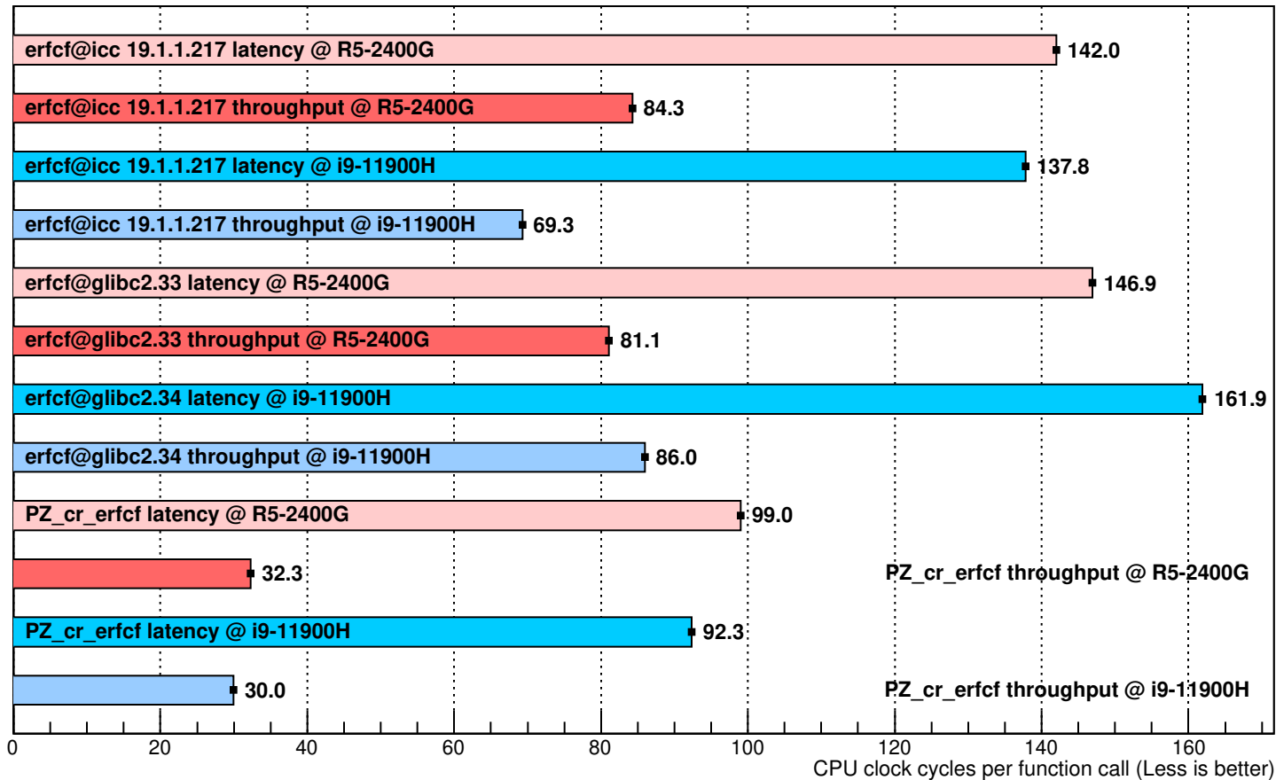
Performance of erfcf implementations (100000 random uniformly distributed arguments in [-4.07, 10.68])
