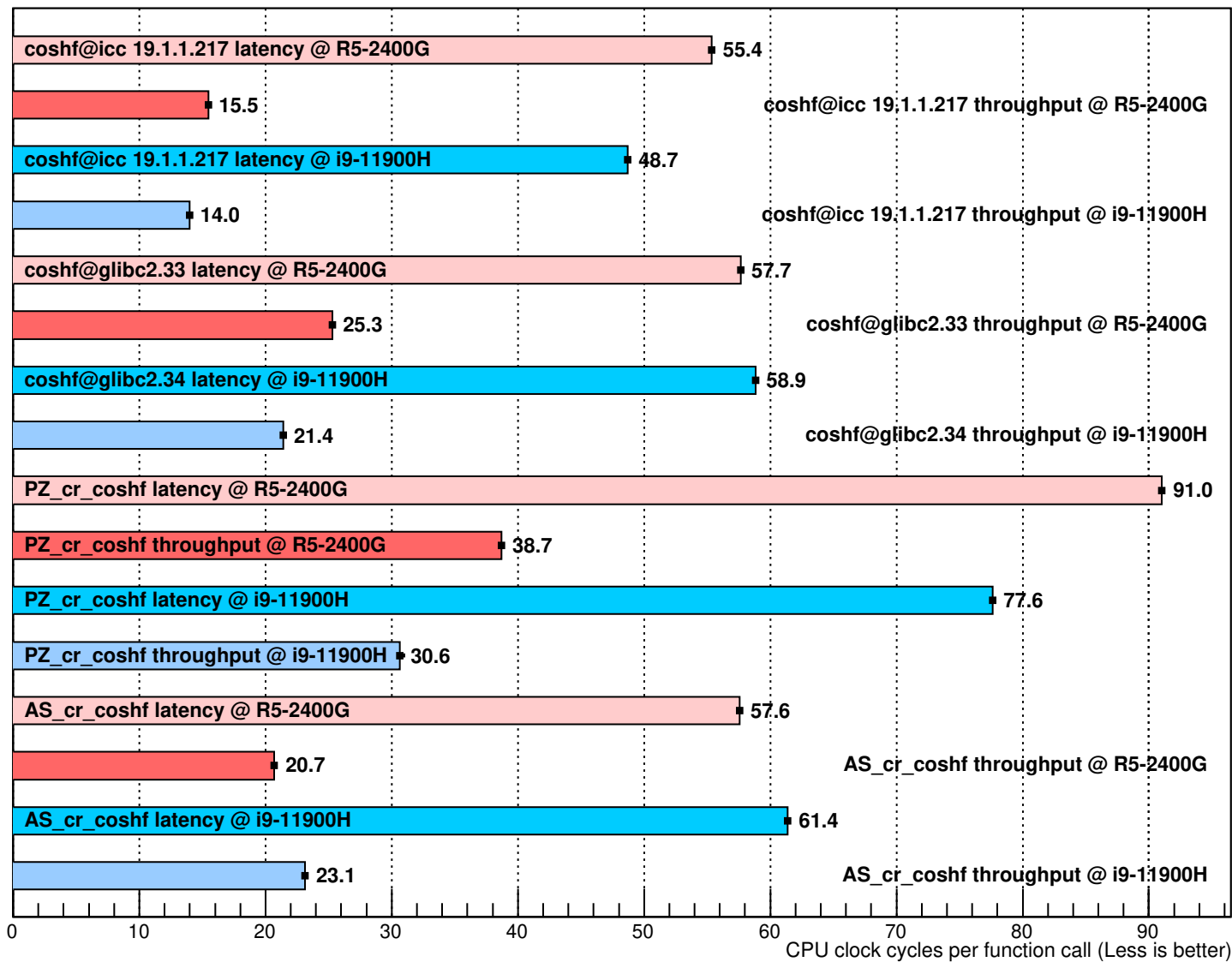
Performance of coshf implementations (10000 random uniformly distributed arguments in [-10, 10])
