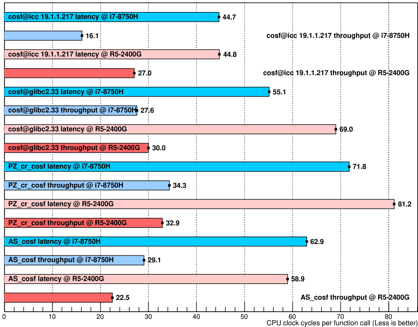
Performance of cosf implementations (10000 random uniformly distributed arguments in [0, 2\pi] )
