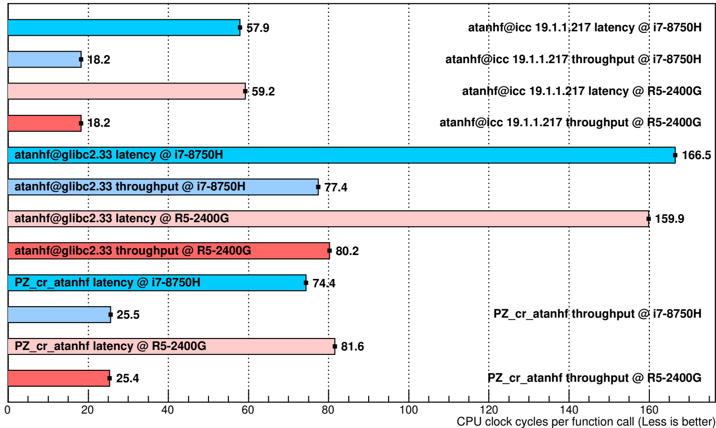
Performance of atanhf implementations (10000 random uniformly distributed arguments in [-1, 1])
