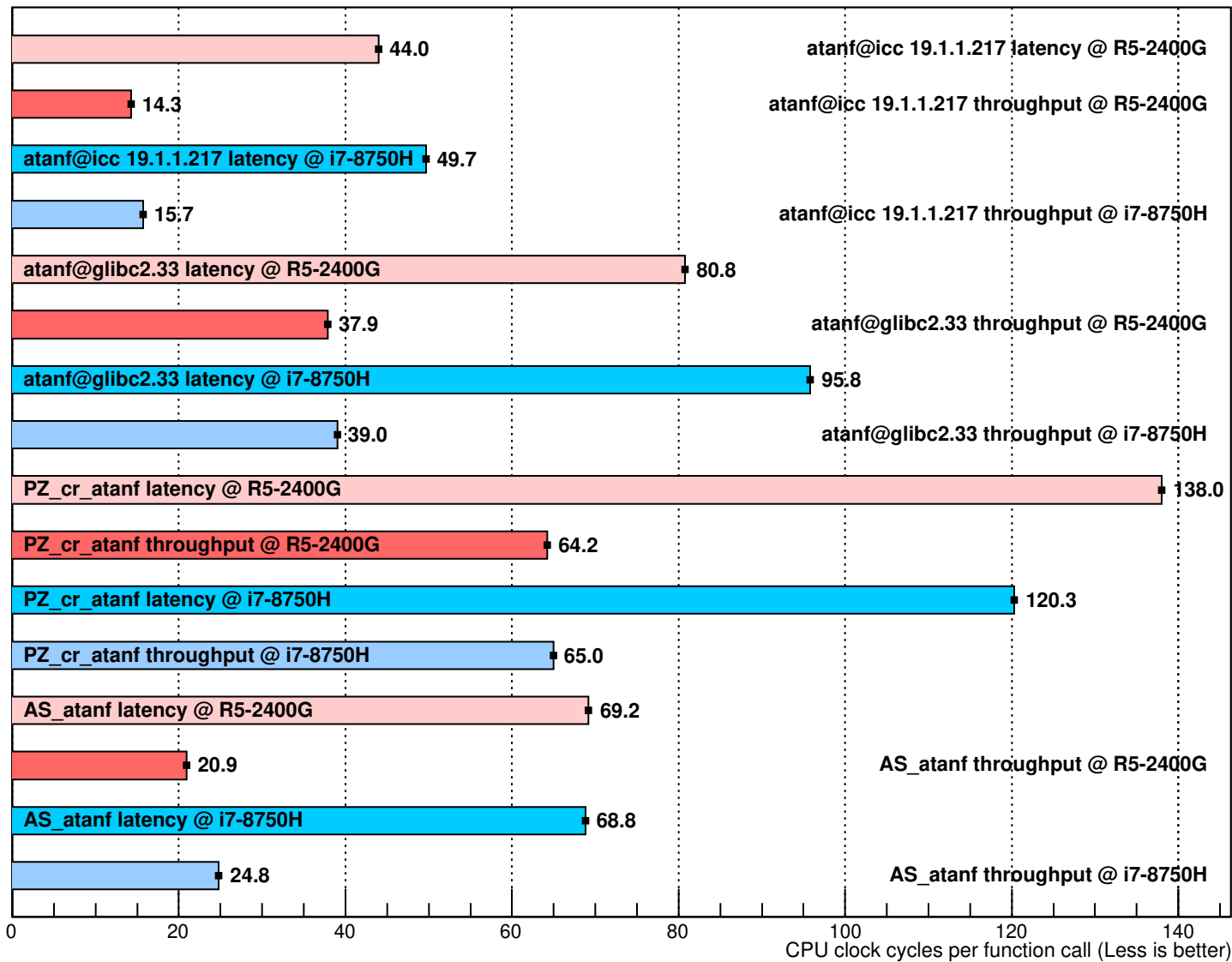
Performance of atanf implementations (10000 random uniformly distributed arguments in [-10, 10])
