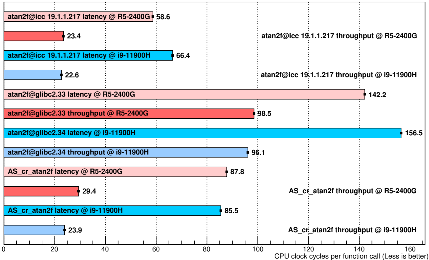
Performance of atan2f implementations (100000 random uniformly distributed arguments in [-10, 10]x[-10, 10])
