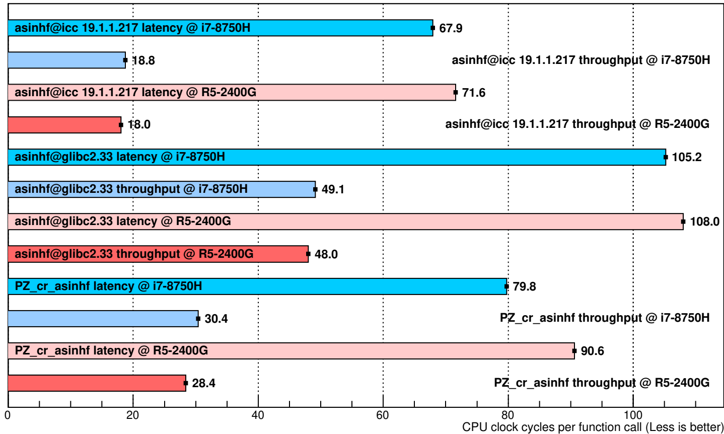
Performance of asinhf implementations (10000 random uniformly distributed arguments in [-10, 10])
