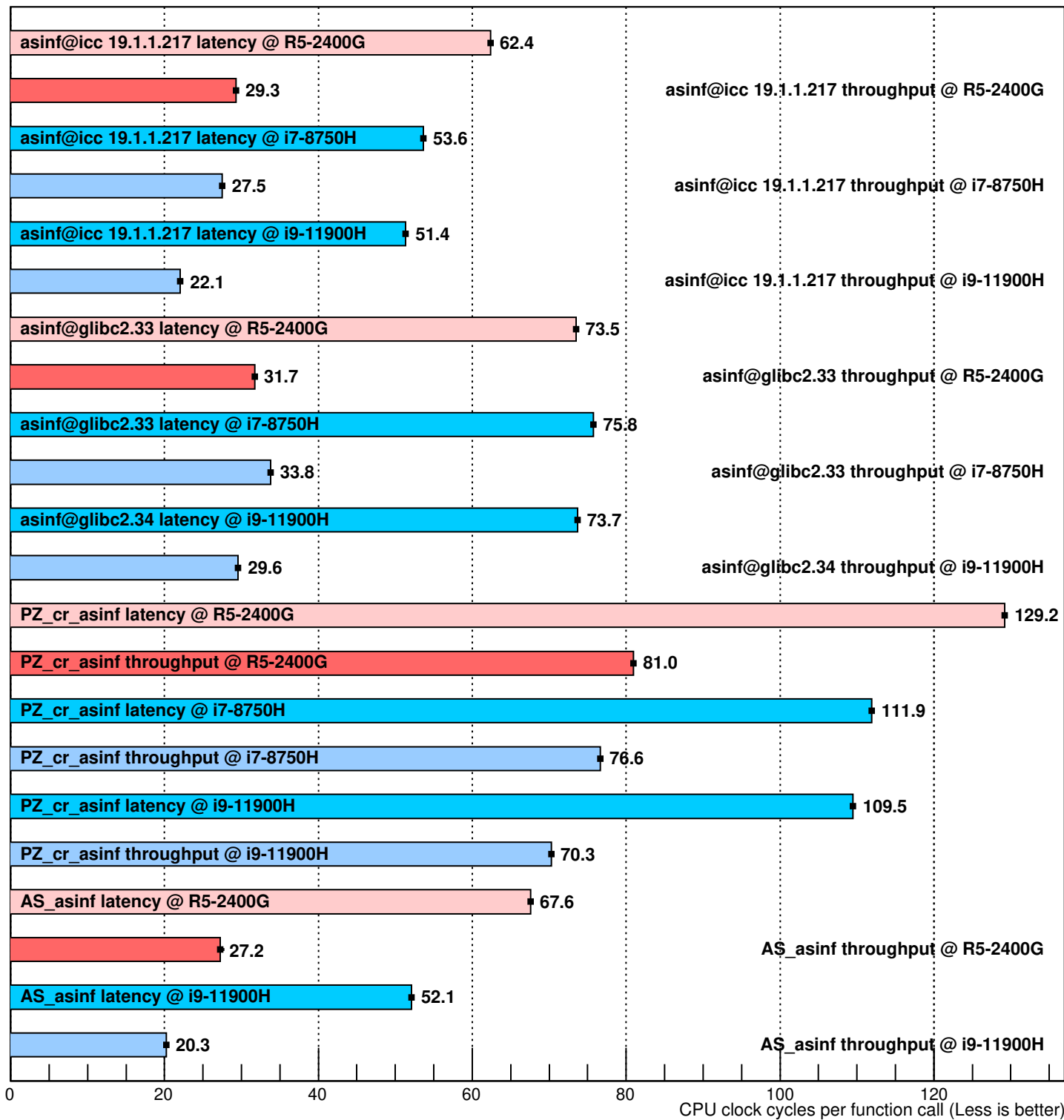
Performance of asinf implementations (10000 random uniformly distributed arguments in [-1, 1])
