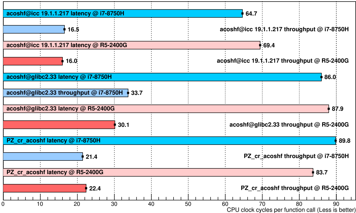
Performance of acoshf implementations (10000 random uniformly distributed arguments in [1, 21])
