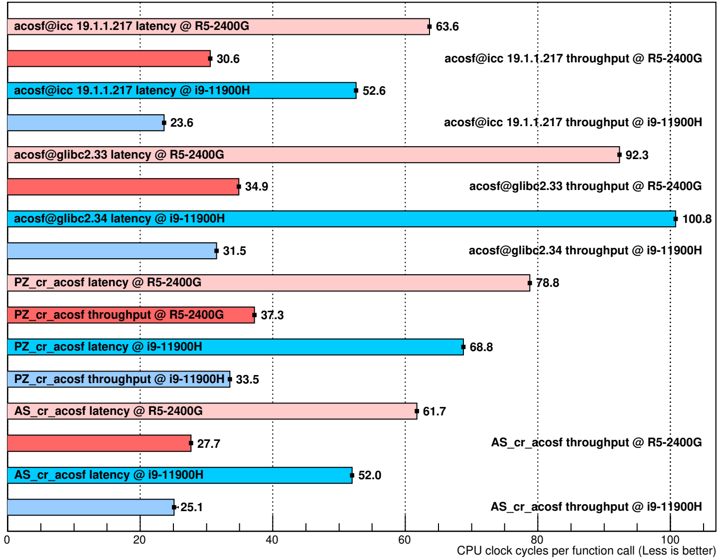
Performance of acosf implementations (10000 random uniformly distributed arguments in [-1, 1])
